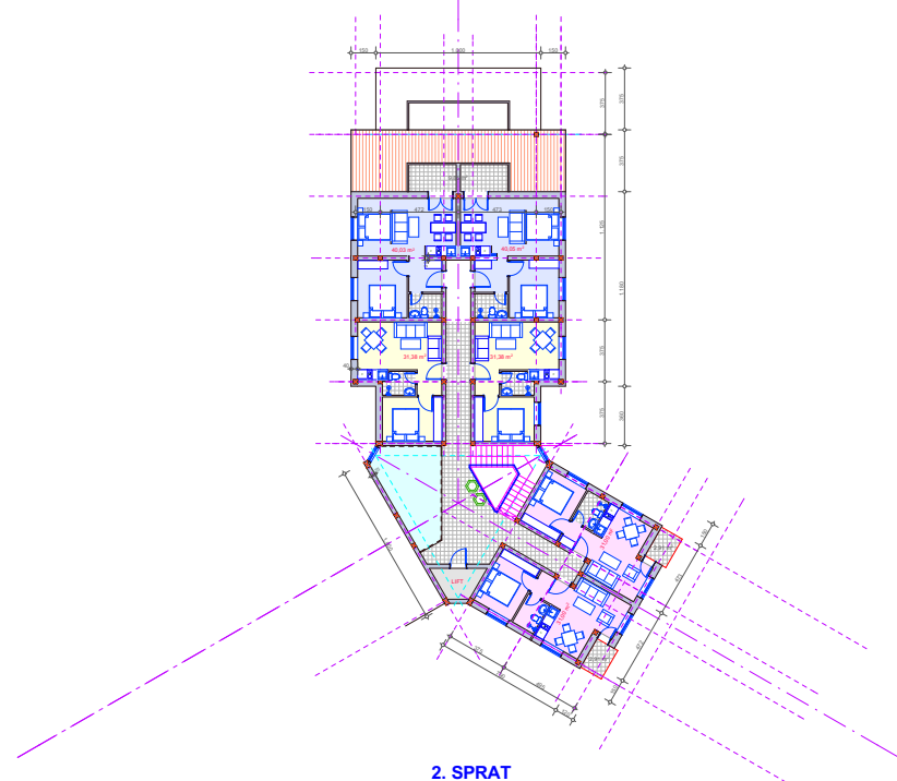
2. SPRAT 6 apartmana (2+4) BRGP=335m 2
